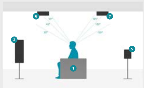
5.1.4 Ceiling Speaker Placement Detail
